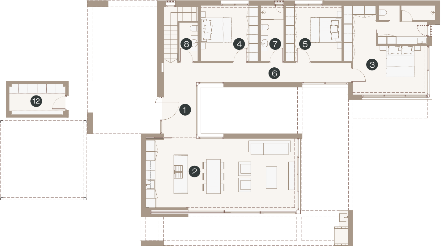
GROUND FLOOR
