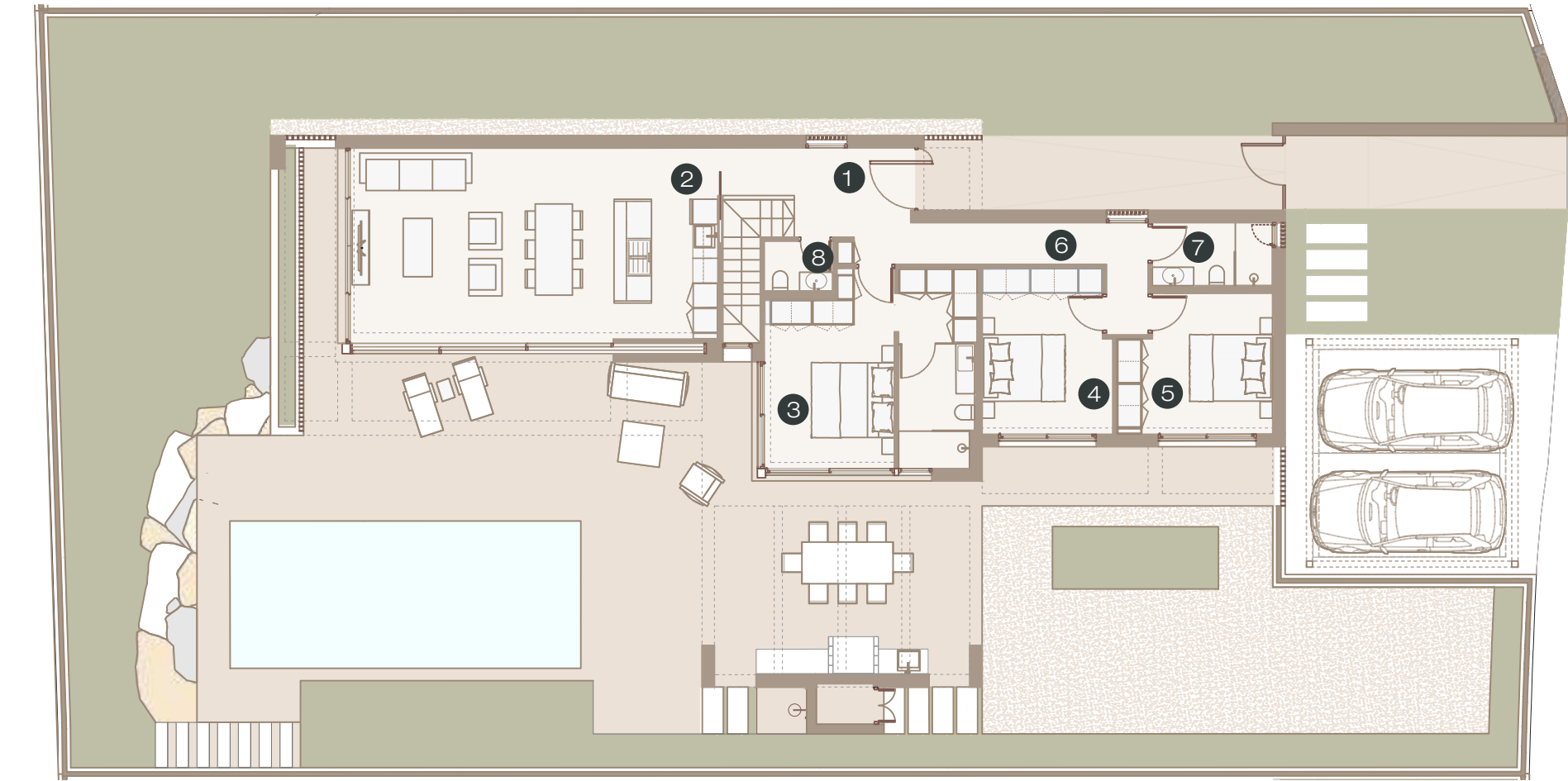
PLOT FLOOR
