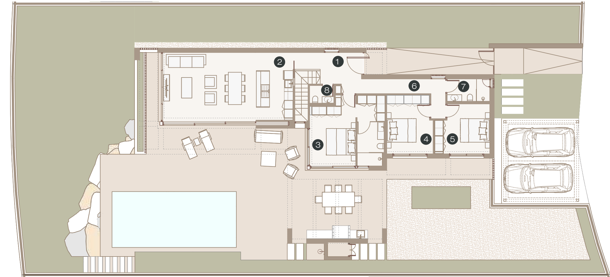
PLOT FLOOR
